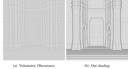
Figure 7: Volumetric obscure vs. our shading. A comparison between a screen-space obscuration algorithm [LS10] (a), and our term (b), which is a mix of directional light, ambient occlusion and line drawing shading.
